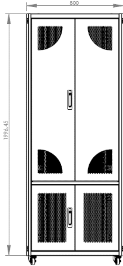
REAR VIEW
