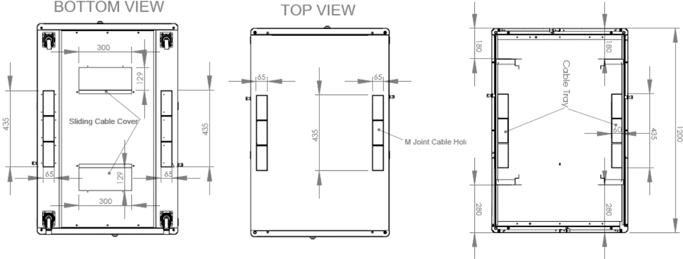
BOTTOM VIEW
