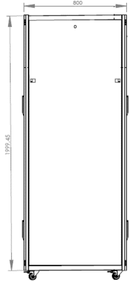
SIDE VIEW
